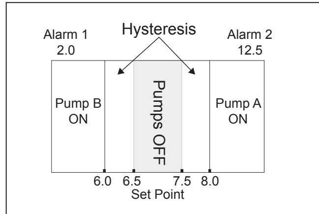
Pump A Control Profile
