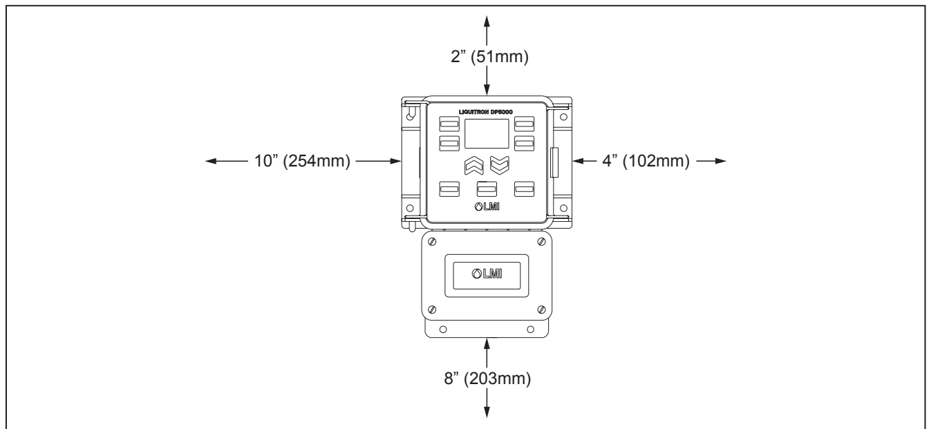
Figure 2. Minimum Clearances
