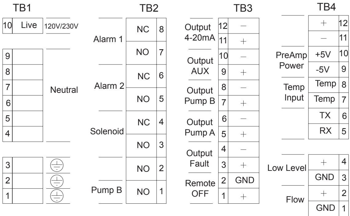
Figure 5. Terminal Strip
