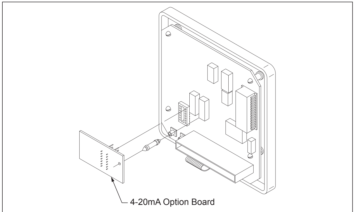
Figure 6. Circuit Board
