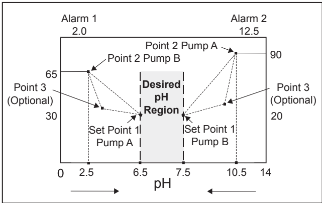
Figure 10. Pump A Control Profile
