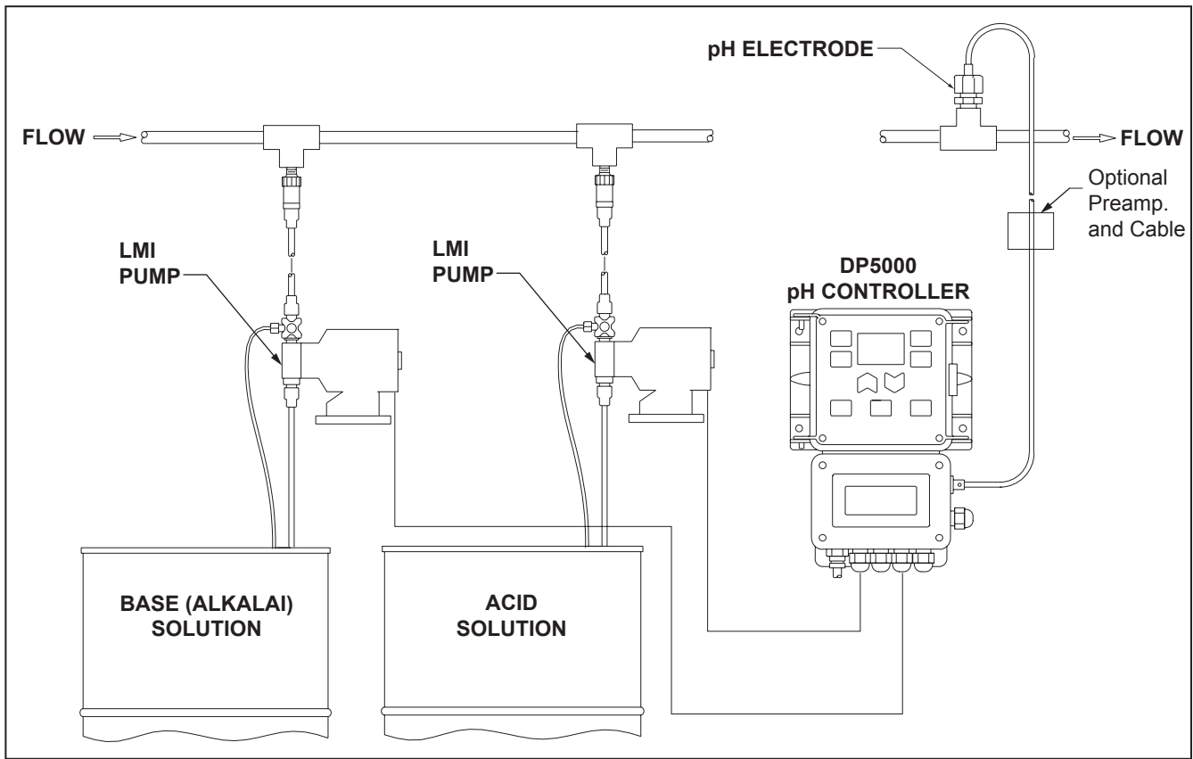
Figure 3A. Typical In-Line Installation
