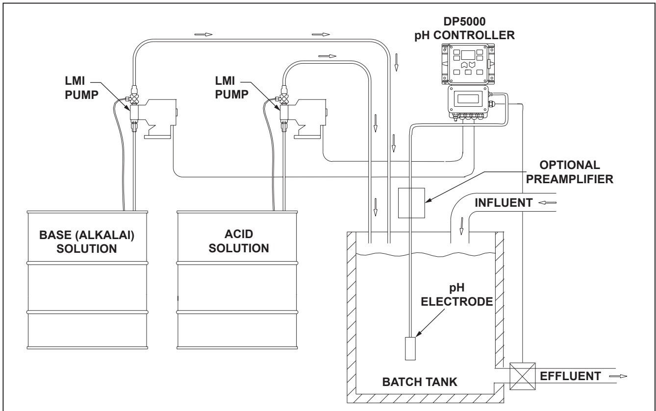
Figure 3B. Typical Batch Installation
