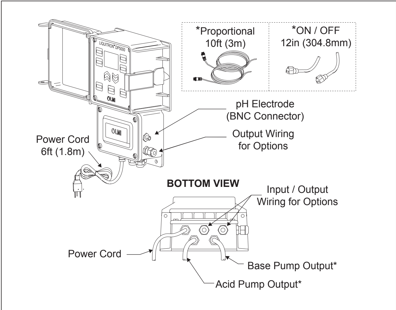
Figure 4. Electrode and Pump Connections
