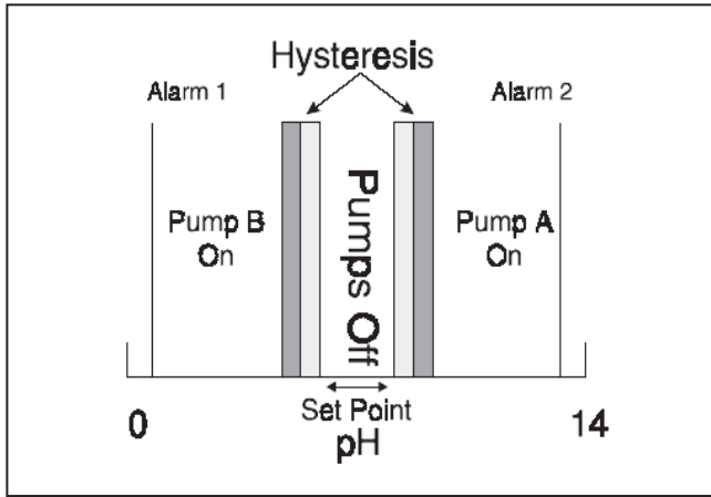
Figure 8. ON / OFF Control
